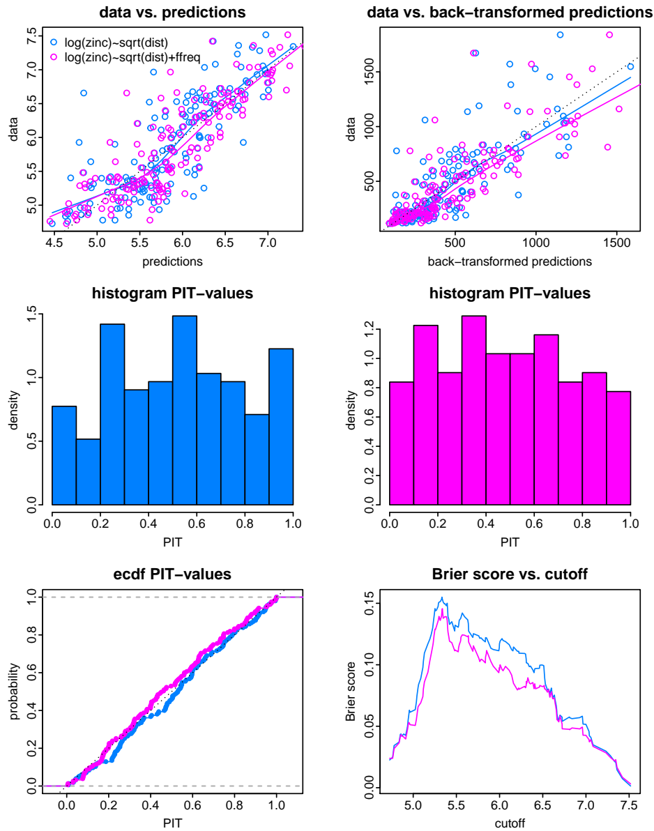
Figure 10: Diagnostic plots of cross-validation predictions of REML fits of models \log(\text{zinc}) \sim \text{sqrt}(\text{dist}) (blue) and \log(\text{zinc}) \sim \text{sqrt}(\text{dist}) + \text{ffreq} (magenta).
