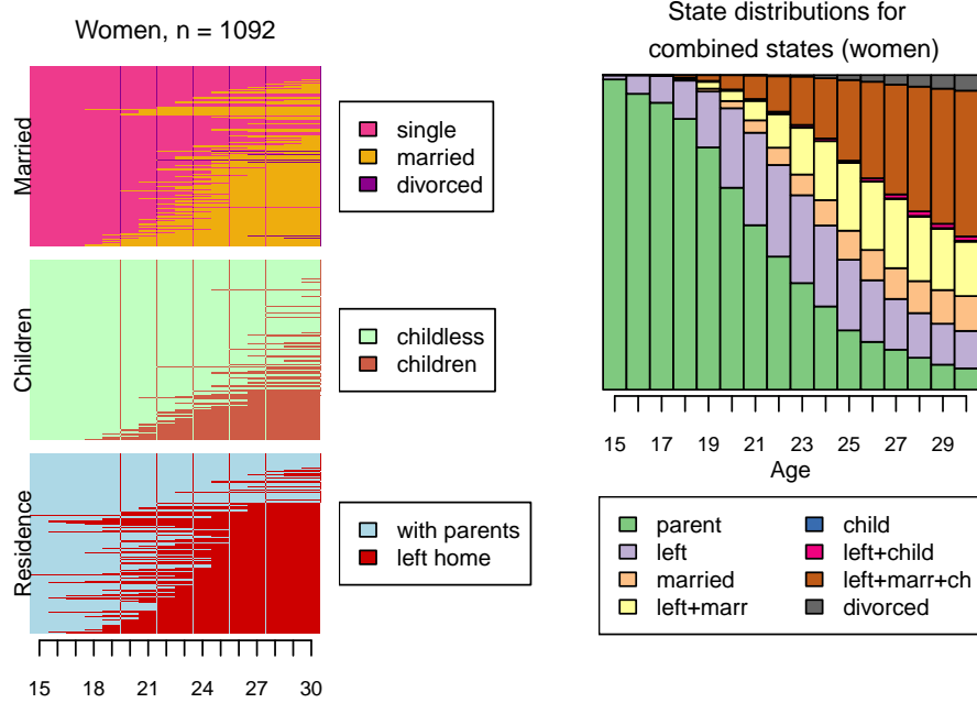
Figure 10: Another example of gridplot . Showing three-channel sequences and state distributions of combined states for women.
