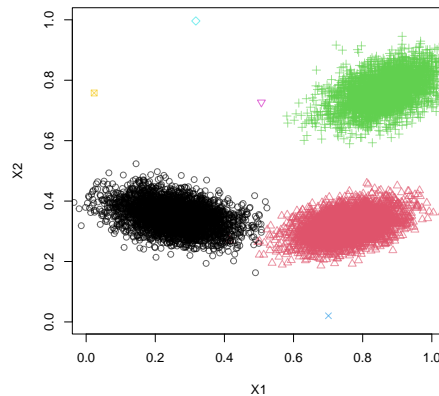
Figure 7: Plotting 10000 data instances from the data stream comprising outliers.
