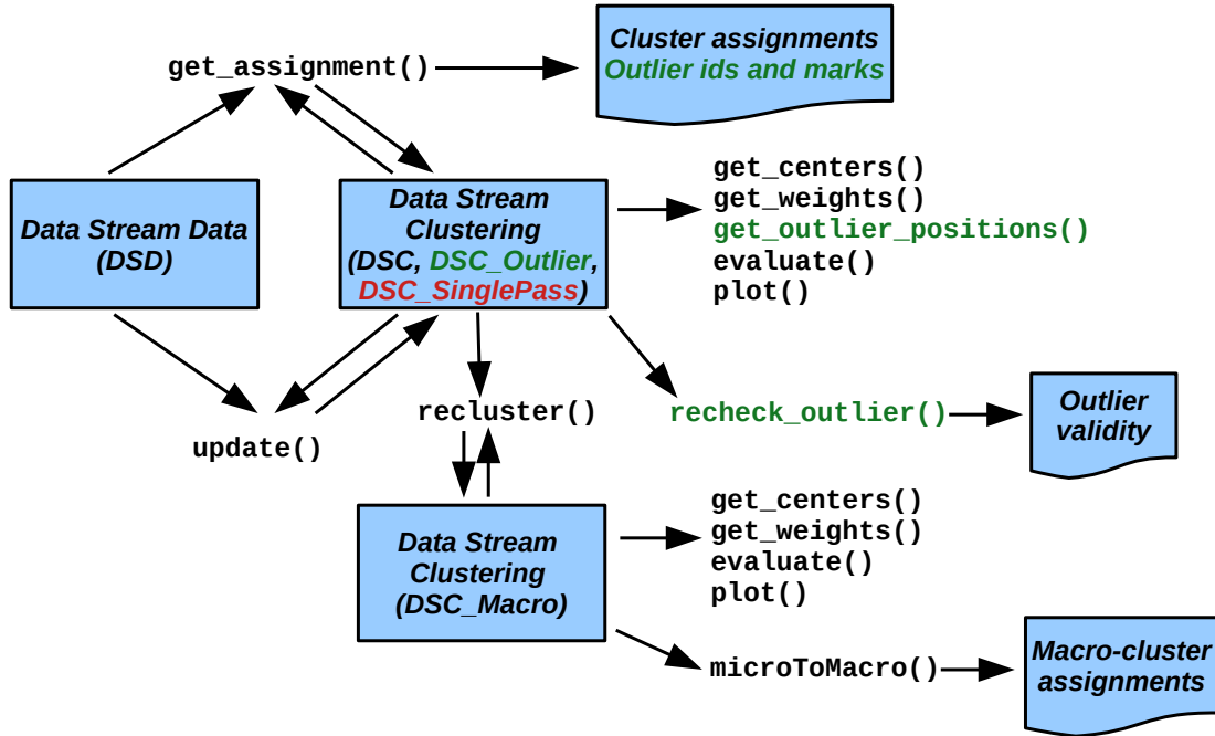
Figure 13: Interaction between the DSD and single-pass / outlier detector DSC classes.
