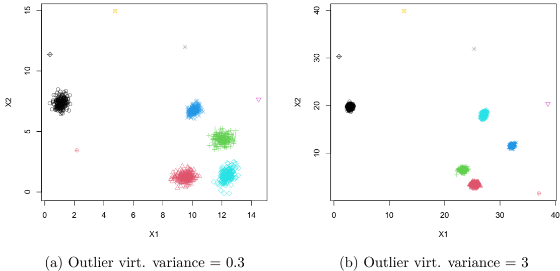
Figure 10: Data points from DSD_Gaussians having distinct outlier virtual variances.
