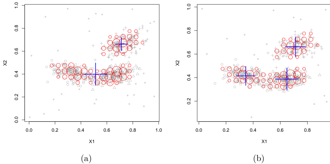
Figure 17: A data stream clustered with D-Stream using the (a) built-in reclustering strategy, and (b) reclustered with weighted k -means and k = 3 .
