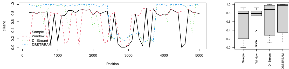
Figure 23: Evaluation of data stream clustering of an evolving stream.
