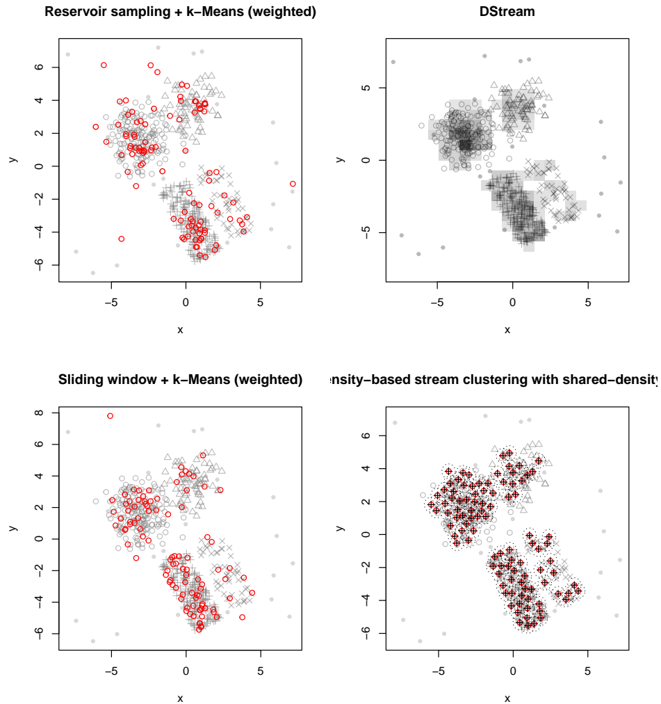
Figure 21: Micro-cluster assignment areas for different data stream clustering algorithms.
