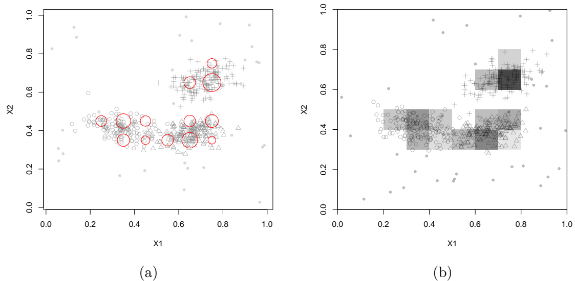
Figure 14: Plotting the micro-clusters produced by D-Stream together with the original data points. Shown as (a) micro-clusters and as (b) dense grid cells.
