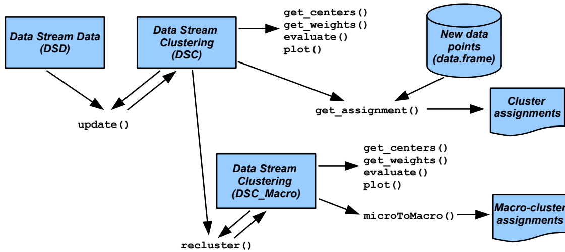
Figure 12: Interaction between the DSD and DSC classes.
