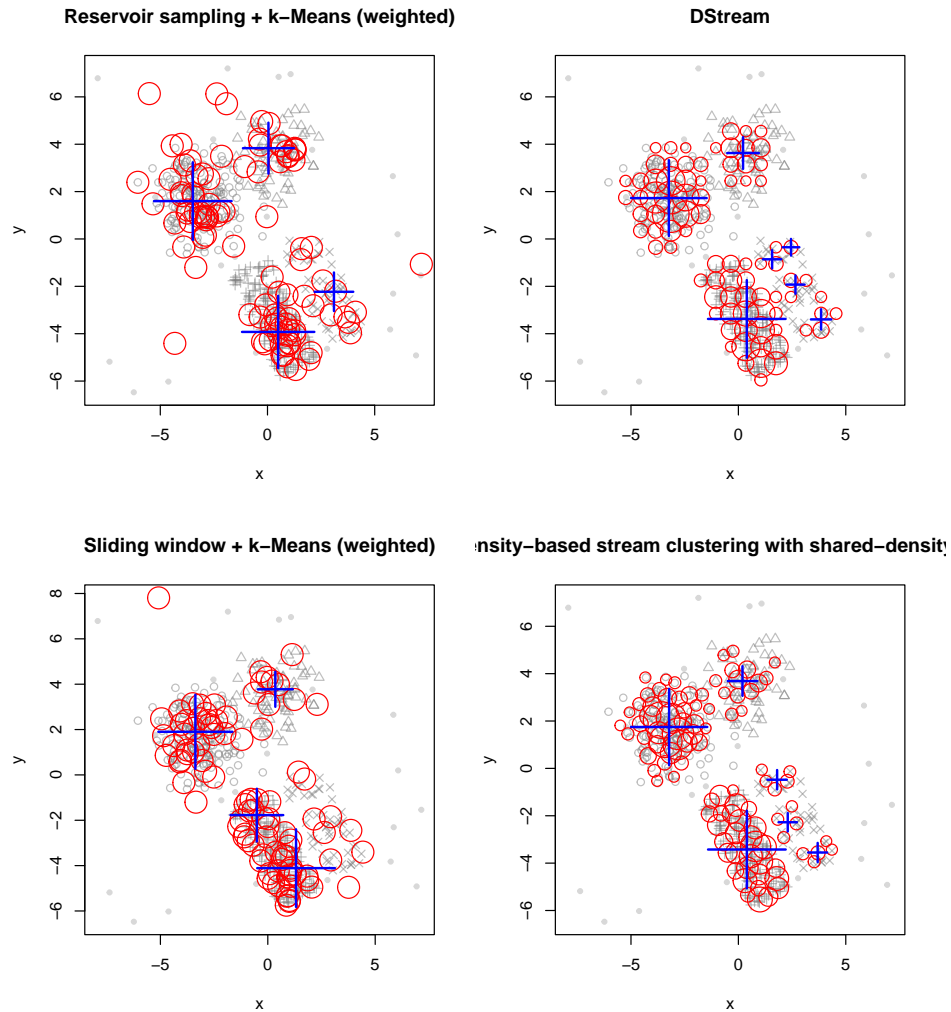
Figure 22: Macro-cluster placement for different data stream clustering algorithms.
