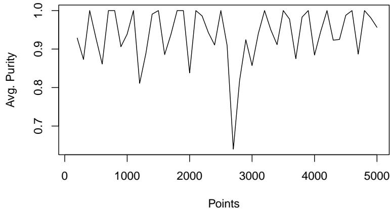
Figure 15: Micro-cluster purity of D-Stream over an evolving stream.
