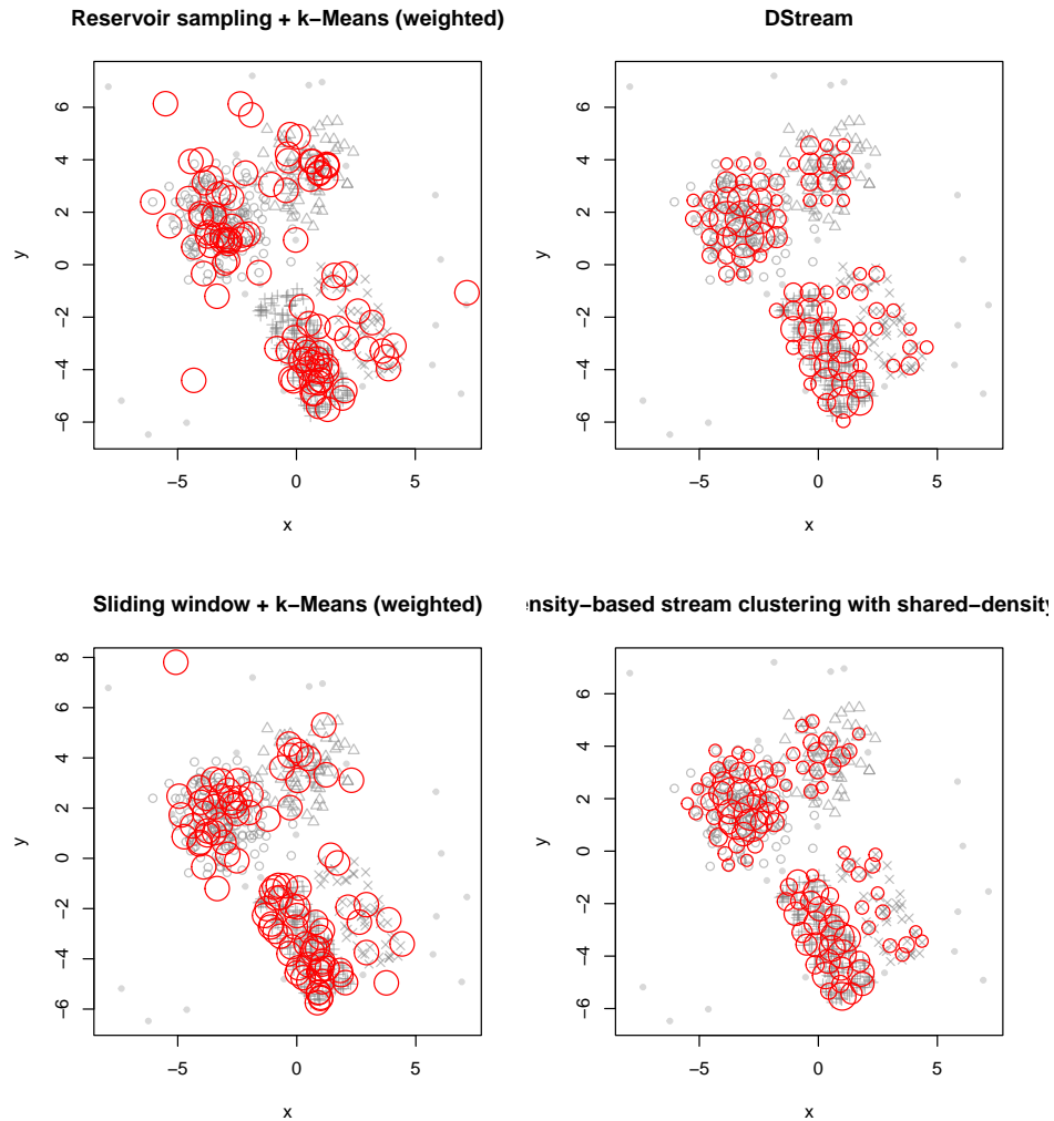
Figure 20: Micro-cluster placement for different data stream clustering algorithms.
