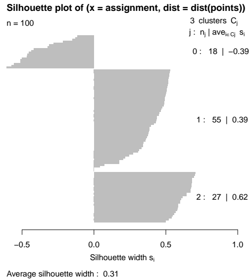
Figure 18: Silhouette plot for D-Stream clustering with two macro-clusters and a cluster ( j = 0 ) representing the unassigned points.
